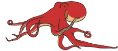
giant Antarctic octopus
